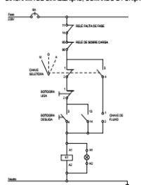
DIAGRAMA UNIFILAR
